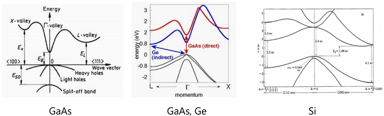
Fig.3. Classification of semiconductors according to the relative position of the valence and conduction band.
