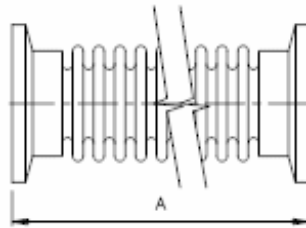
Flange with Hose nozzle, Flexible Bellows with Flanges 5.3.2. Vacuum clamps according to ISO-K DIN 28404
