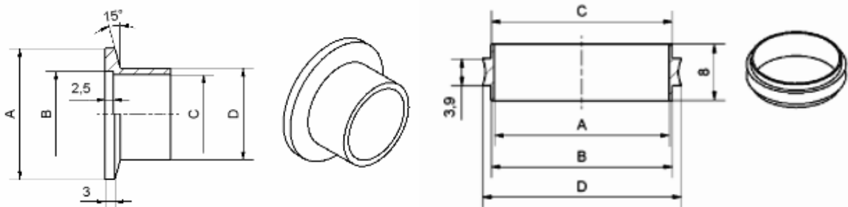
Flanges with tabulation, Centering Rings
