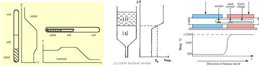
Fig.8. Bridgman method
