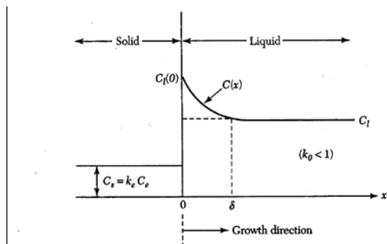
Doping distribution near the solid-melt interface.
