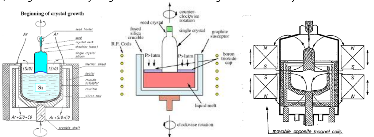
Fig.4. Czoehralski growth of Si, LEC CZ growth of GaAs, Mixing of the melt by Eddy currents
