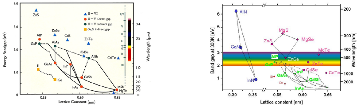
Fig.2. Classification of semiconductors according to the position in the periodic table, to the width of the forbidden gap and to the lattice constant, respectively.
