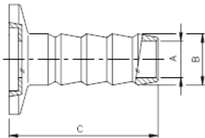
Flange with Hose nozzle, Flexible Bellows with Flanges 5.3.2. Vacuum clamps according to ISO-K DIN 28404
