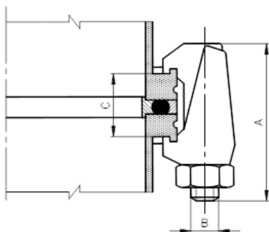
Flange with Hose nozzle, Flexible Bellows with Flanges 5.3.2. Vacuum clamps according to ISO-K DIN 28404
