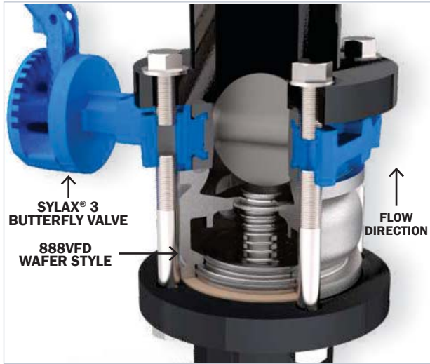
Shown with Flomatic® Model 888S6VFD wafer check valve close coupled with Sylax®3 butterfly valve. Butterfly valve can be operated with check valve in an “open” or “closed” position with no interference.
