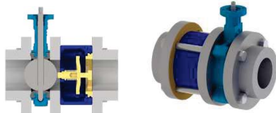
Shown with Flomatic® Model 888S6VFD wafer check valve close coupled with Sylax®3 butterfly valve. Butterfly valve can be operated with check valve in an “open” or “closed” position with no interference.
