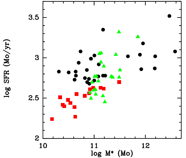
Fig. 10. The star formation rate (SFR) obtained from the far infrared luminosity, versus the stellar mass of galaxies in our sample (full black circles), compared to the sample of Da Cunha et al (2010, full red squares) and Fiolet et al (2009, full green triangles).
