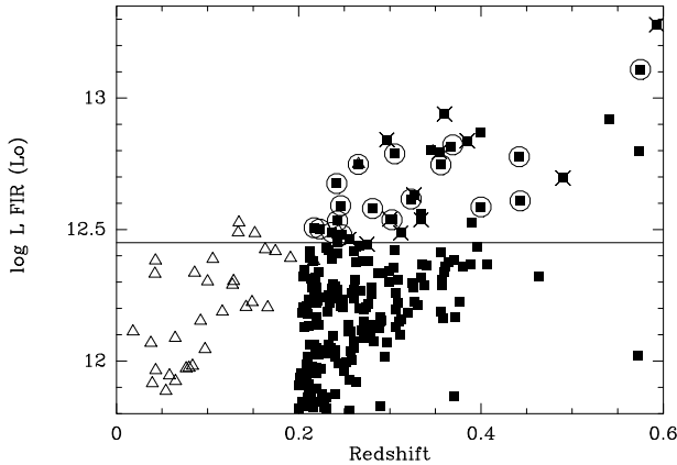
Fig. 1. Definition of our sample. Among the 209 northern galaxies (filled symbols) found in NED between 0.2 < z < 0.6 and detected at 60\mu\text{m} by IRAS, we selected the most luminous ones ( \log L_{\text{FIR}}/L_{\odot} > 12.45 , as indicated by the horizontal line). By comparison, the ULIRGs in the sample of Solomon et al. (1997) are plotted as open triangles. The circles indicate detections, non-detections are marked by a cross. Sources that have neither a circle nor a cross could not be observed due to weather conditions.
