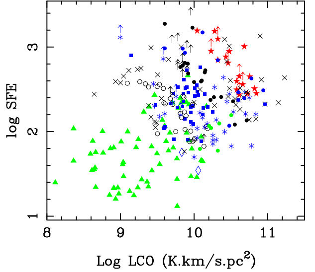
Fig. 9. Star formation efficiency \text{SFE} = L_{\text{FIR}}/M(\text{H}_2) , versus CO luminosity, assuming the same CO-to- \text{H}_2 conversion factor \alpha = 0.8 M_{\odot} (\text{K km s}^{-1} \text{pc}^2)^{-1} . All symbols are as defined in Fig 6.
