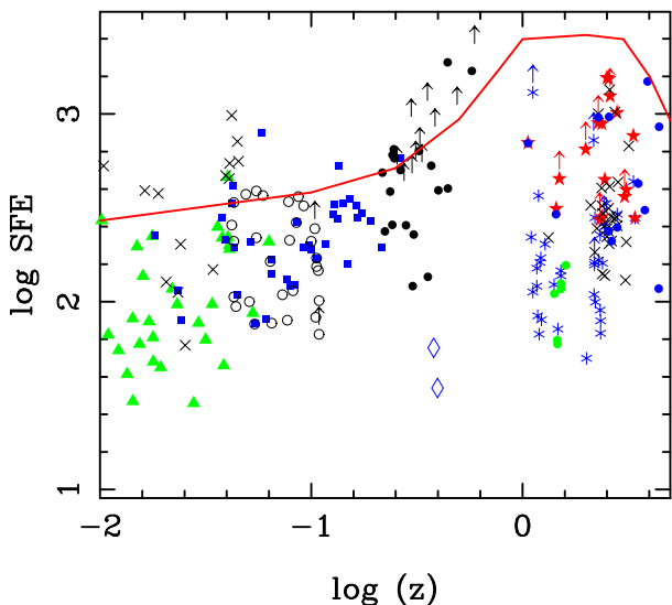
Fig. 13. Same as Figure 9, but versus redshift. The red curve is a schematic line summarizing the cosmic star formation history, from the compilation by Hopkins & Beacom (2006), complemented with the GRB data by Kistler et al. (2009) and the optical data from Bouwens et al. (2008). The red curve is logarithmic and only indicative of relative variations of the star formation rate per cubic Mpc as a function of redshift, and can be translated vertically.
