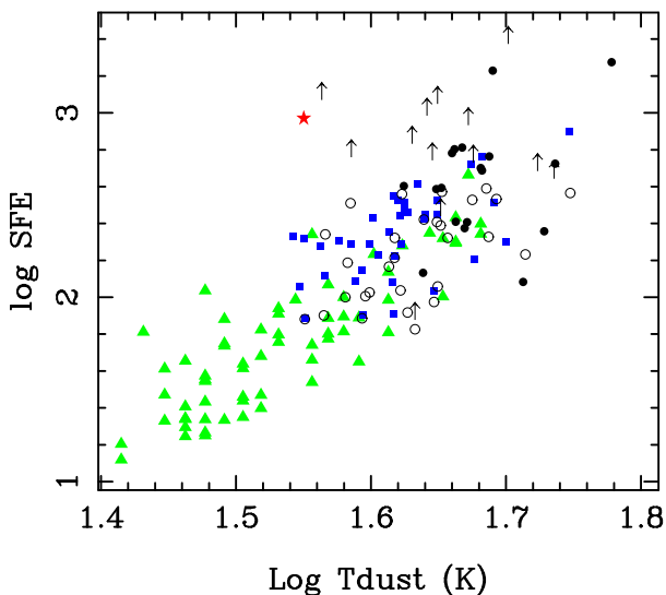
Fig. 12. Same as Figure 9, but versus T_d , for the sources where it could be defined. For the submillimeter galaxies, the red star corresponds to the averaged SFE, with the mean dust temperature of 35.5 found by Kovacs et al. (2010).
