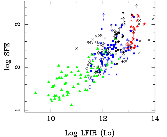
Fig. 11. Same as Figure 9, but versus L_{\text{FIR}} .
