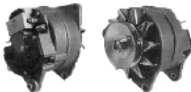
18-5975 Alternator Replaces: Perkins 2871A651 Valeo 2939590 Motorola 9AR3959G, 3855G, 6000G, 510-845, -860, -864 (28 Volt 45 AMP) For Perkins Marine Engine: 6-354-4, SAEJ1171
