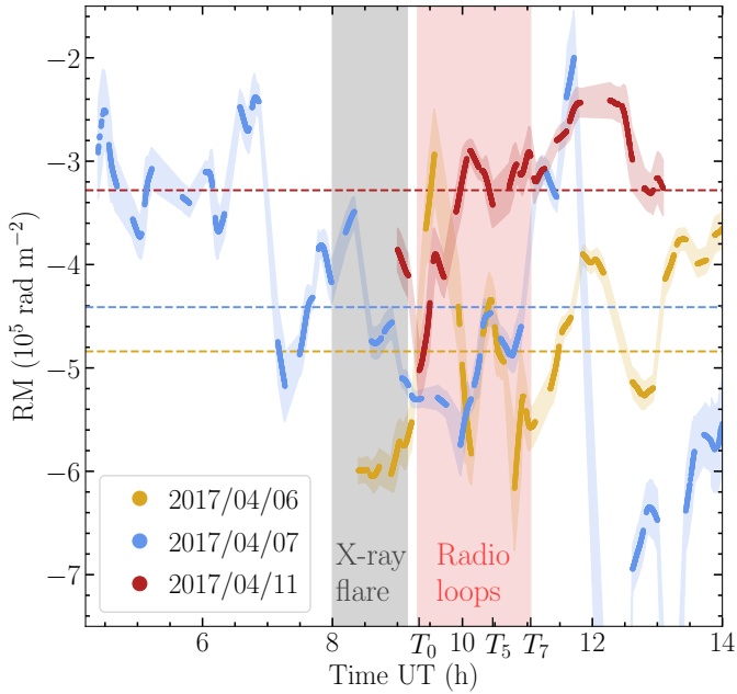
Fig. A.1. Rapid variation of the RM at millimeter wavelengths in Sgr A*. The plot corresponds to the RM fit with linear regression across all four bands on 4 s cadence, smoothed with a Gaussian filter with 6 min standard deviation, with color bands around the mean RM indicating the local signal standard deviation. Dashed lines represent the mean daily values reported by Goddi et al. (2021). We observe rapid swings of the RM on timescales \sim 0.5 h, indicating a presence of the intrinsic Faraday screen component corresponding to the innermost region of the accretion flow. The vertical gray and red bands indicate the time range of the X-ray flare and polarimetric loops observed on 2017 Apr 11.
