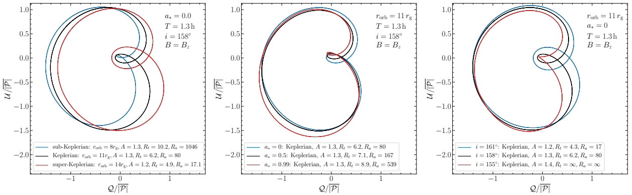
Fig. C.1. Impact of modifying parameters of the fiducial model: Keplerianity and orbital radius with a fixed orbital period (left), black hole spin (center), and inclination (right). The presence and size of the small inner loop puts strong constraints on the inclination and orbital radius admitted by the vertical magnetic field model. Additionally, in the vertical magnetic field model framework, the observed loop size may suggest a large positive spin of Sgr A*.
