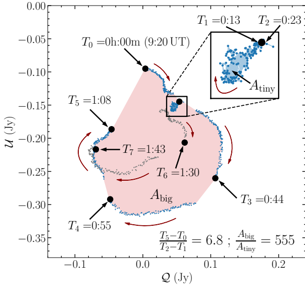
Fig. 2. Polarimetric loops observed by ALMA at 229 GHz on 2017 Apr. 11. The observations began at T_0 = 9:20 UT (MJD 57854.39), 30 min after the peak of the X-ray flare. We highlight the small inner loop A_{\text{tiny}} . Following the full loop A_{\text{big}} between T_0 and T_5 , a similar pattern continues between T_5 and T_7 , with a decreased period and reduced LP.
