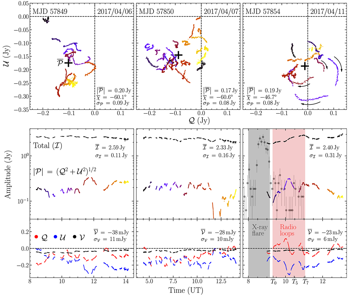
Fig. 1. Full Stokes 229 GHz ALMA light curves of Sgr A* obtained on 2017 Apr. 6, 7, and 11. Top row: linear polarization represented on a Q – U plane. The color of the curve indicates the time from the beginning of the observation. Crosses “+” show the locations of the daily mean linear polarization \bar{\mathcal{P}} with the EVPA \bar{\chi} . The pattern observed on 2017 Apr. 11 suggests the presence of coherent clockwise Q – U loops, emphasized with arrows. Bottom rows: full Stokes Sgr A* light curves. On Apr. 11, ALMA started observing immediately after the X-ray flare (gray band region). Chandra X-ray data are plotted in counts per second and were arbitrarily scaled. The red-shaded region corresponds to the period in which polarimetric loops are apparent.
