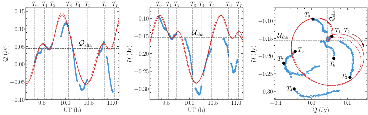
Fig. 3. Comparison between ALMA data in the loopy period on 2017 Apr. 11 (blue dots) and hot spot model prediction for the inclination i = 158^\circ , the orbital radius r_{\text{orb}} = 11 M , the vertical magnetic field, and the spin a_* = 0 . We compare predictions of a simplified semi-analytic model (dashed red lines, Appendix B and Gelles et al. 2021) with a slow light, full radiative transfer model (continuous red line, Vos et al. 2022). A static, linearly polarized component of |\mathcal{P}_{\text{sha}}| = |Q_{\text{sha}} + iU_{\text{sha}}| = 0.16 Jy and \chi_{\text{sha}} = -37^\circ was coherently added to the hot spot models, and the loop position angle was adjusted to match the observations.
