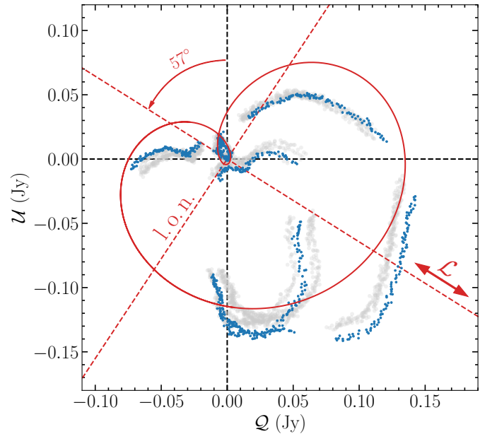
Fig. F.1. Intrinsic LP in the loopy period, after removing the mean effect of the Faraday rotation. The 229 GHz band data are shown with a blue color, while the three remaining ALMA frequency bands are shown with a gray color. The implied PA of the line of nodes (l.o.n.) of the hot spot orbit as seen in the sky was estimated at about 147^\circ east of north. The intrinsic PA of the hot spot angular momentum \mathcal{L} was found to be \sim 57^\circ east of north (or 227^\circ , given the 180^\circ ambiguity).
