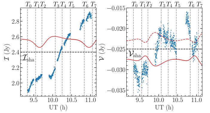
Fig. E.1. Total intensity \mathcal{I} and circular polarization \mathcal{V} comparison between the fiducial hot spot model presented in Fig. 3 and the observations. A static source with a total intensity of \mathcal{I}_{\text{sha}} = 2.4 \text{ Jy} and a circular polarization of \mathcal{V}_{\text{sha}} = -0.025 \text{ Jy} , representing the contribution from the observable black hole shadow, was added to the model. For circular polarization, we show the results corresponding to two opposite magnetic field orientations (red continuous and dashed lines).
