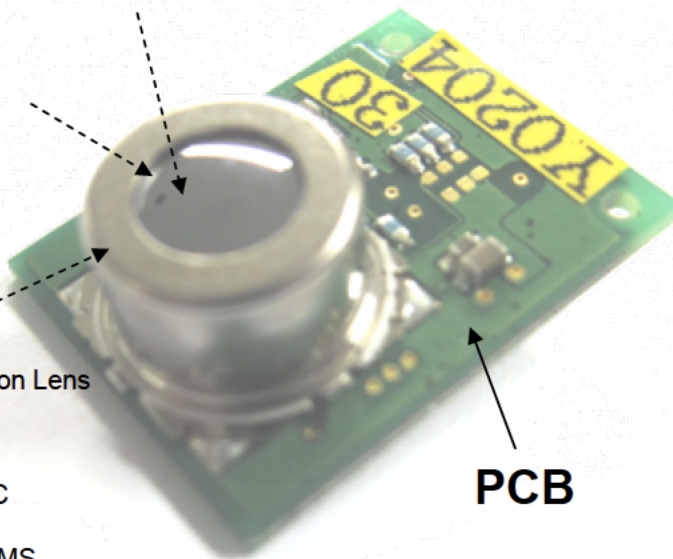
Thermopile
