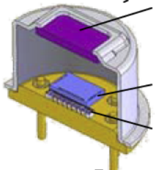
Thermopile
