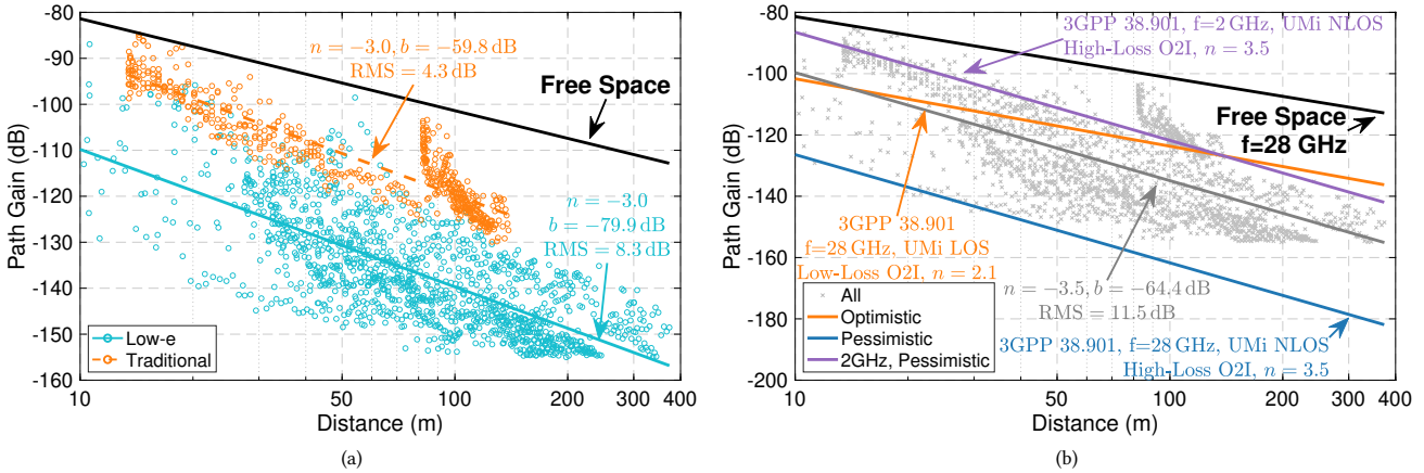
Figure 4: Models for glass: (a) models for “traditional” and Low-e glass calculated from OI scenario clusters, (b) comparison of the path gain model for the cluster of all OI scenarios to optimistic and pessimistic models developed from 3GPP UMi path loss predictions for different types of glass.
