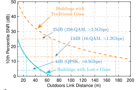
Figure 10: 10 th percentile SNR predictions for buildings with Low-e or traditional glass windows, with coverage ranges d^* labeled for various MCS.
