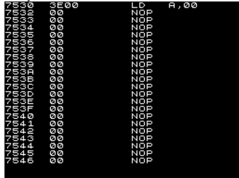
Disassembler (Gary Stimson,1989) Utility: Assembler/Disassembler/Monitor
