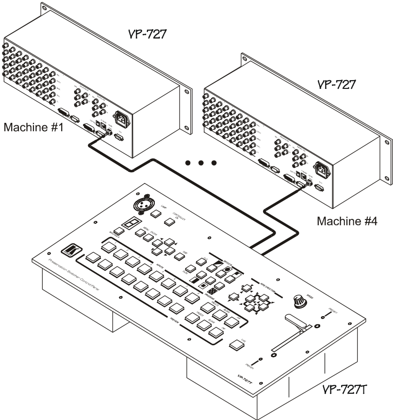
Figure 7: Connecting the VP-727T
