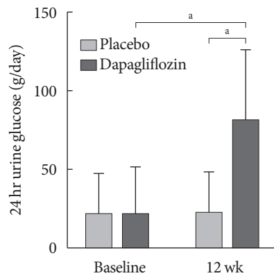
Supplementary Fig. 2. Twenty-four hour urine glucose excretion. Values are presented as mean \pm standard deviation. a P < 0.05 .
