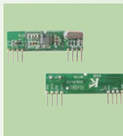
RF Super Heterodyne 3400 Receiver Module (MU002)
