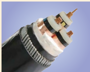
Medium Voltage Swa Armoured Power Cable (YJV32)
