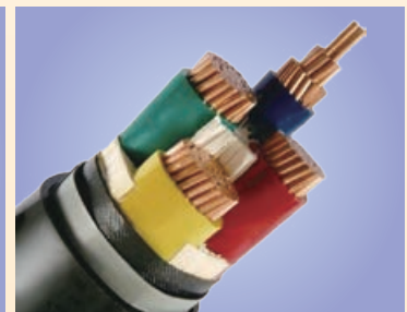
Low Voltage XLPE Insulated Swa Armoured Power Cable (YJV22)
