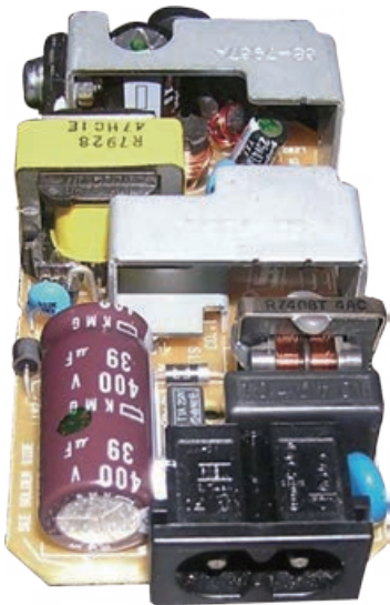
PCBA for Various Power Supplies (PCBA-PS)
