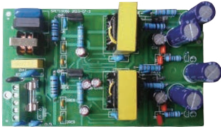
PCBA for Constant Current Power Supplies
