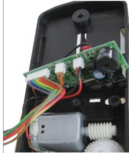
PCBA for Electronic Door Locks
