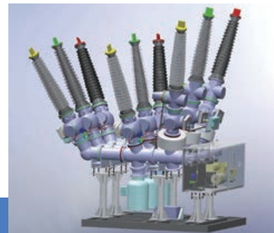
Hybrid Gas Insulated Switchgear (ZHW)
