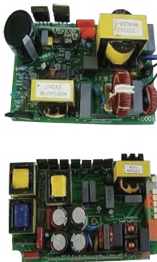
PCBA for Electronic Ballasts (PCBA-B)
