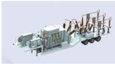
Mobile Substation (132KV)
