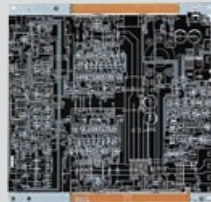
FR-1 PCB 01
