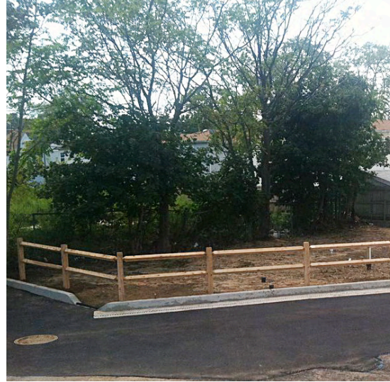
Figure 1-1: Stormwater chambers were installed prior to filling with soil for the construction of a constructed wetland at a DOT parking lot in Far Rockaway. The wetland area, to be planted in Spring 2012, will allow runoff to infiltrate directly into the subsurface system. The adjacent parking lot is paved with porous pavement and excess flow will be directed to the constructed wetland.
