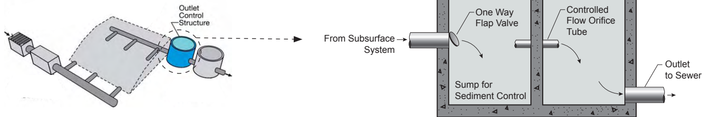
Figure 3-7: The double chamber control structure provides a sump before the controlled flow orifice tube to prevent clogging and an overflow to prevent flooding onsite.
