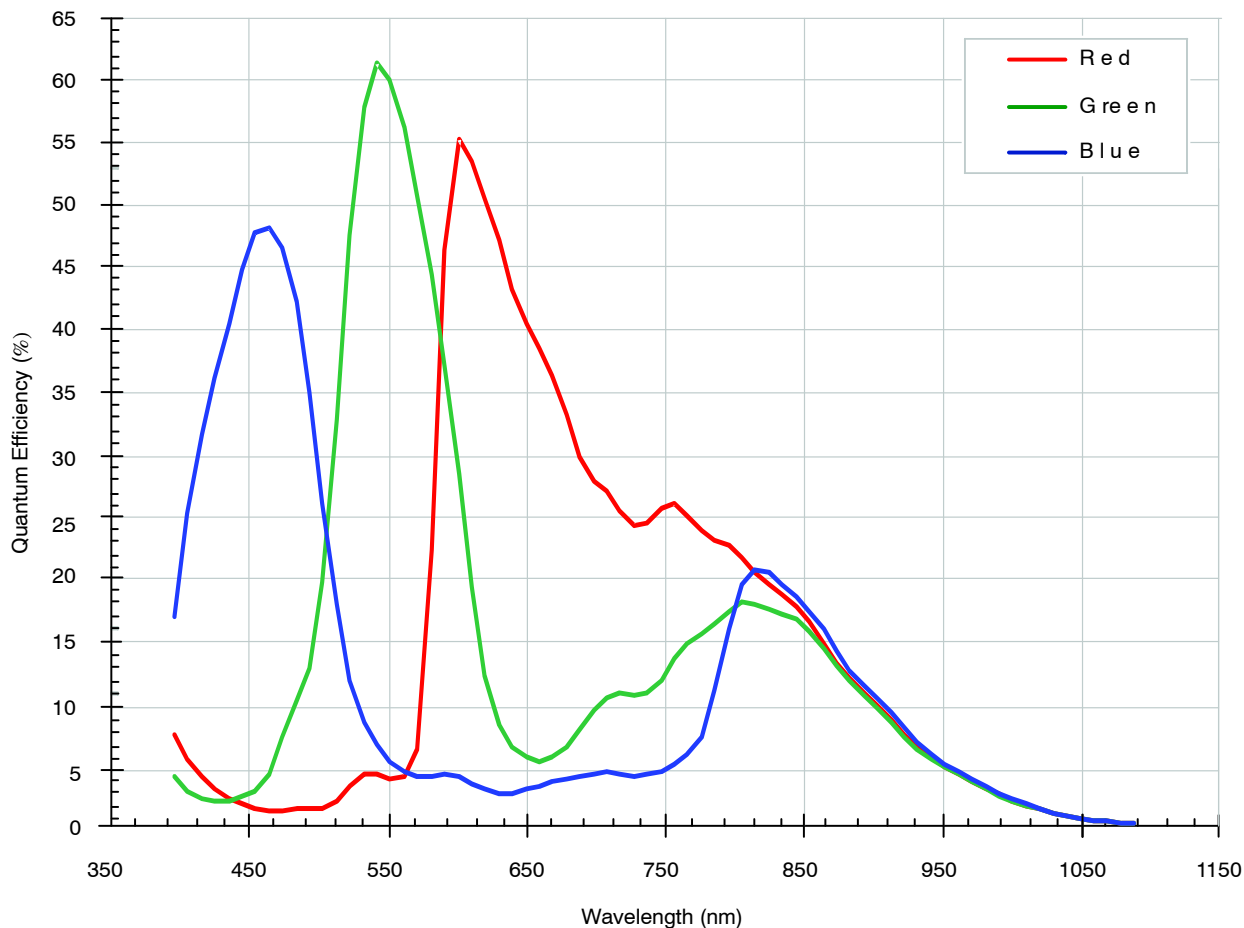
Figure 43. Quantum Efficiency
