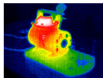
Thermal image
