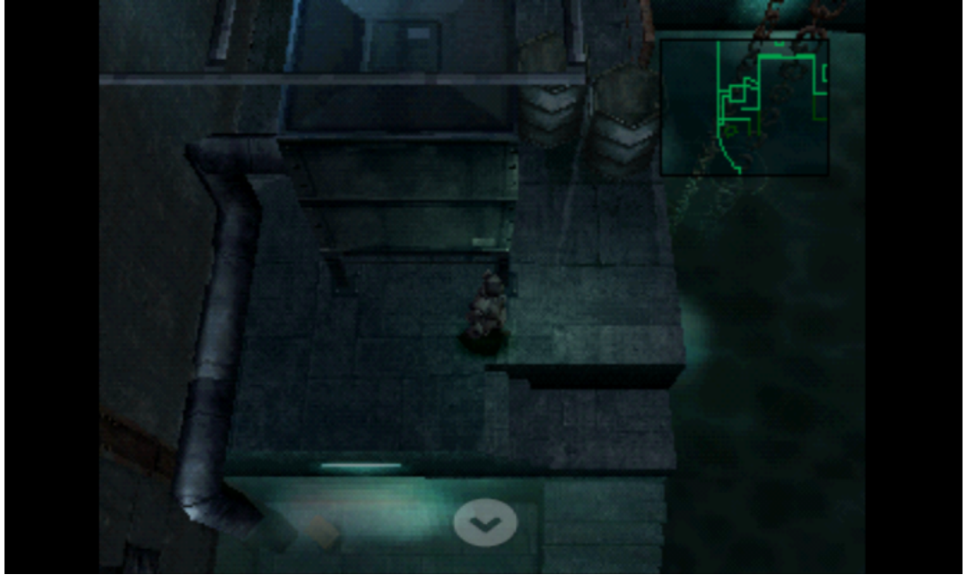
Figure 5: 'Gameplay' screen.
