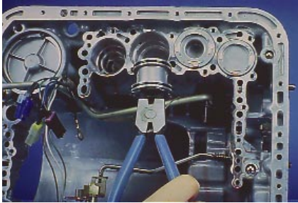
Accumulator Operation
