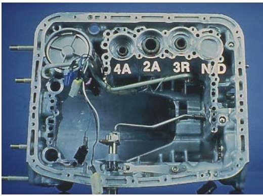
Accumulators
