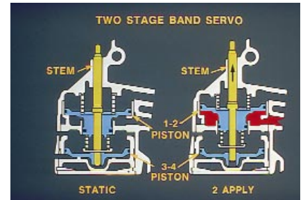
Servo Operation I (later 4EAT models)
