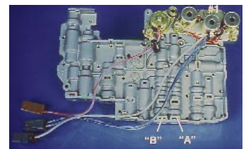
Shift Solenoids 1 and 2
