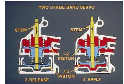
Servo Operation II (later 4EAT models)
