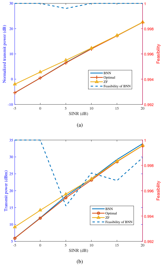
Fig. 8. The power performance averaged over the feasible sample set of the BNN solution in two different cases: (a) without large-scale fading and (b) with large-scale fading under \{K = 4, N = 6\} .
