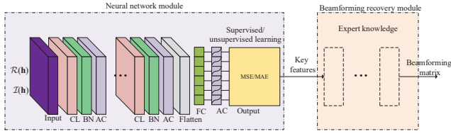
Fig. 1. A DL-based framework for the beamforming optimization in MISO downlink, which includes two main modules: the neural network module and the beamforming recovery module. The neural network module is composed of an input layer, convolutional (CL) layers, batch normalization (BN) layers, activation (AC) layers, a flatten layer, a fully-connected (FC) layer, and an output layer, whereas the key features and the functional layers in the beamforming recovery module are specified by the expert knowledge.
