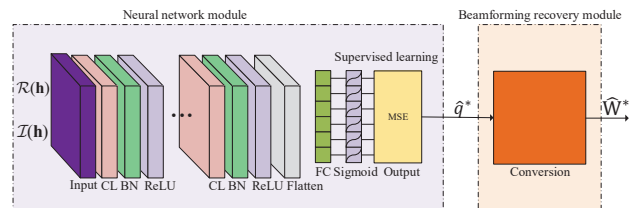
Fig. 3. BNN for the power minimization problem.
